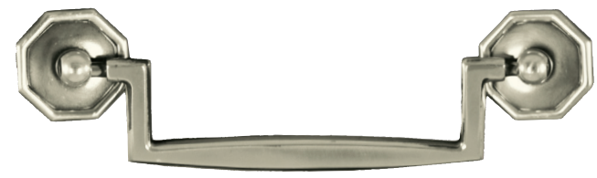
Bail Pull R W 5\frac{3}{4} D \frac{9}{16} H 2\frac{11}{16} (Boring 4\frac{1}{2} )
